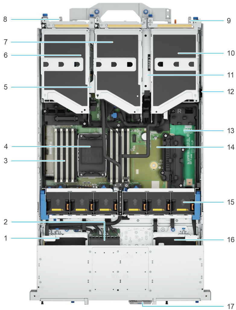
Figure 18. Inside the system with risers
