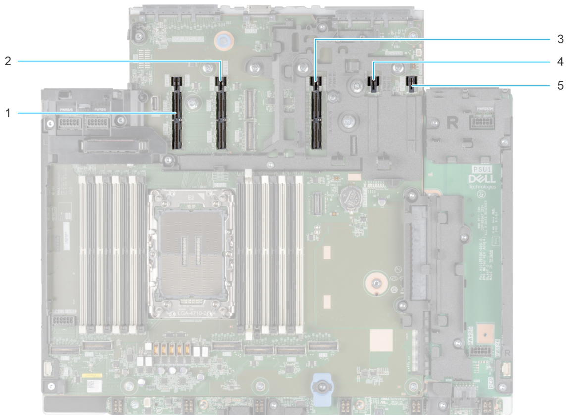
Figure 23. Riser connector location on HPM board
